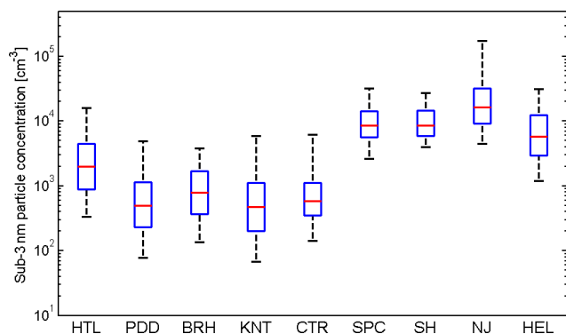
Figure 2. The variation in sub-3 nm particle concentration at different measurements sites. The red lines show the medians, the blue boxes indicate the 25th and 75th percentiles, and the vertical bars show the 5th and 95th percentiles.
