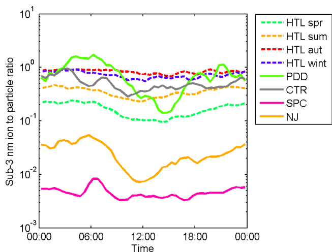
Figure 8. The median diurnal variation in the ratio of sub-3 nm ion concentration to the total particle concentration during different measurement campaigns. The data from Hyytiälä (HTL) are divided into different seasons: spring (spr), summer (sum), autumn (aut), and winter (wint).
