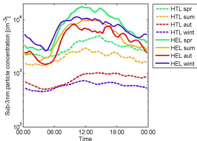
Figure 5. The median diurnal variation in sub-3 nm particle concentration in Hyytiälä (HTL; dashed lines) and in Helsinki (HEL; solid lines) in different seasons: spring (spr), summer (sum), autumn (aut), and winter (wint).
