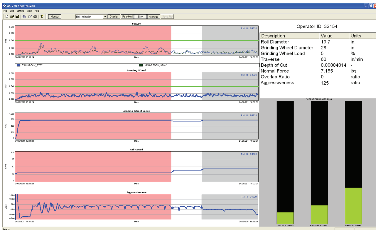
Typical Operator Display Provides Current Grinding Status Including Force, Aggressiveness, Roll/Wheel Speeds, Headstock and Tailstock Vibration
